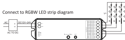
Connect to RGB+CCT LED strip diagram
